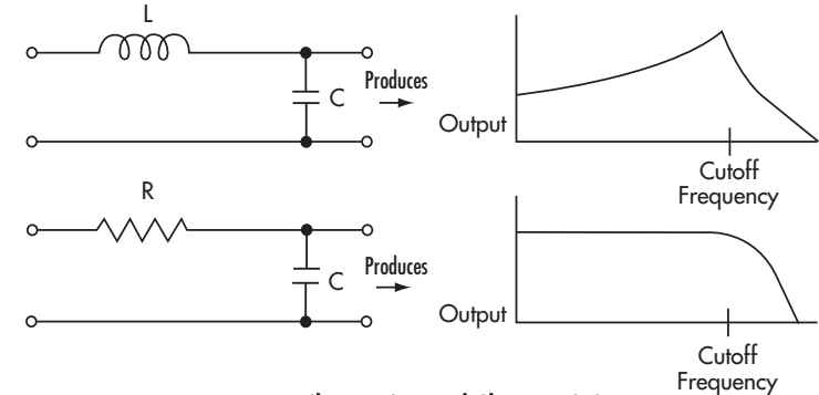
Low Pass Filter Design and Characteristics
