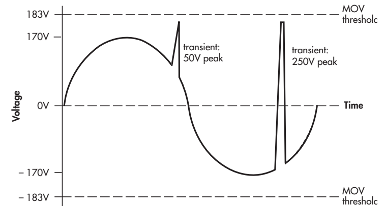
Figure 26: Example of Impulses Not Clamped
