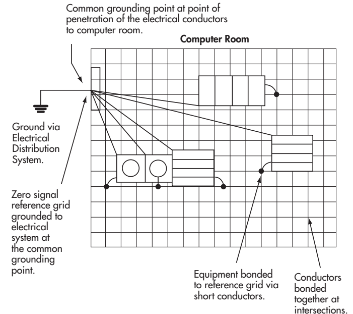
Figure 32: Signal Reference Structure or “Grid”
