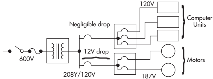
Figure 29: Motor and Computer Loads Supplied from Separate Feeder
