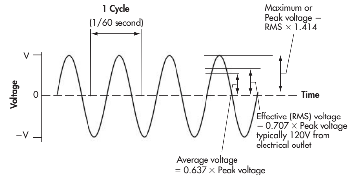
Figure 1: Pure Sinusoidal AC Voltage Waveform
