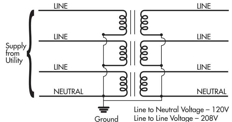
Figure 5: Typical 208 V Three-phase Wye Connected Service
