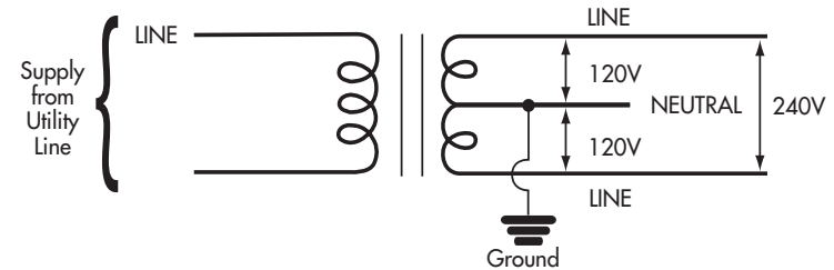
Figure 4: 120/240 V Single-phase Service
