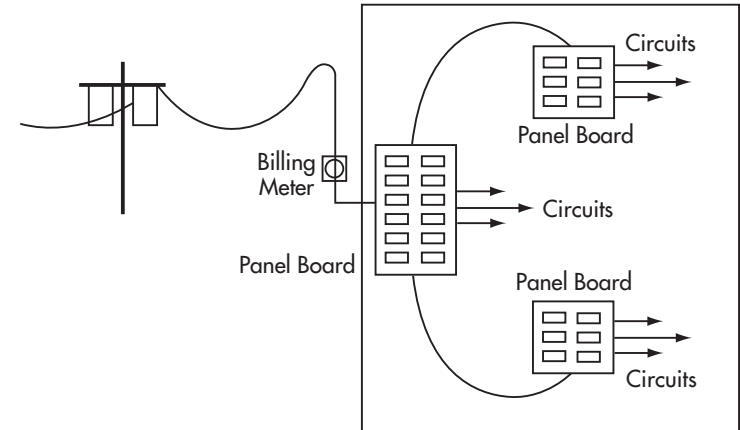
Figure 8: Service with Branch Panel Boards
