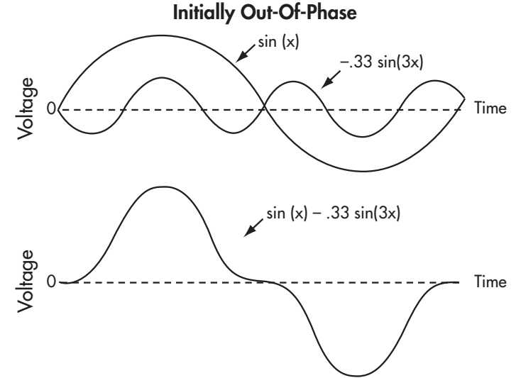
Figure 15: Superposition of Harmonic on Fundamental: Initially Out-of-Phase
