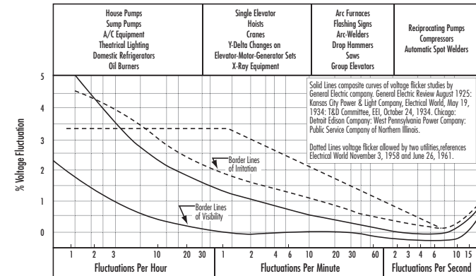
Figure 19: Flicker Curve IEEE 519-1992
